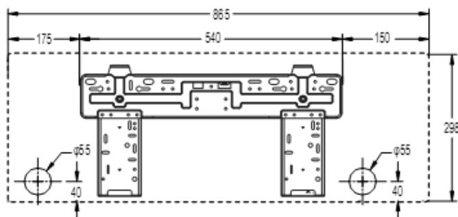
18K Wall Mounting Frame
