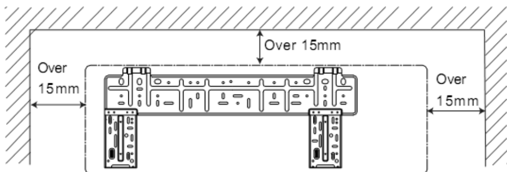
18K Wall Mounting Frame
