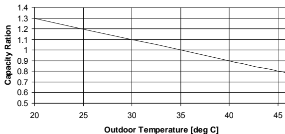
Cooling Capacity Ratio Vs. Outdoor Temperature
